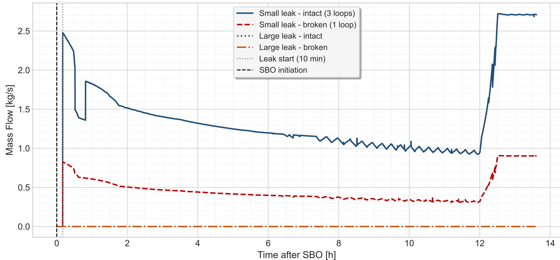
Base Case - RCP Seal Leaks
